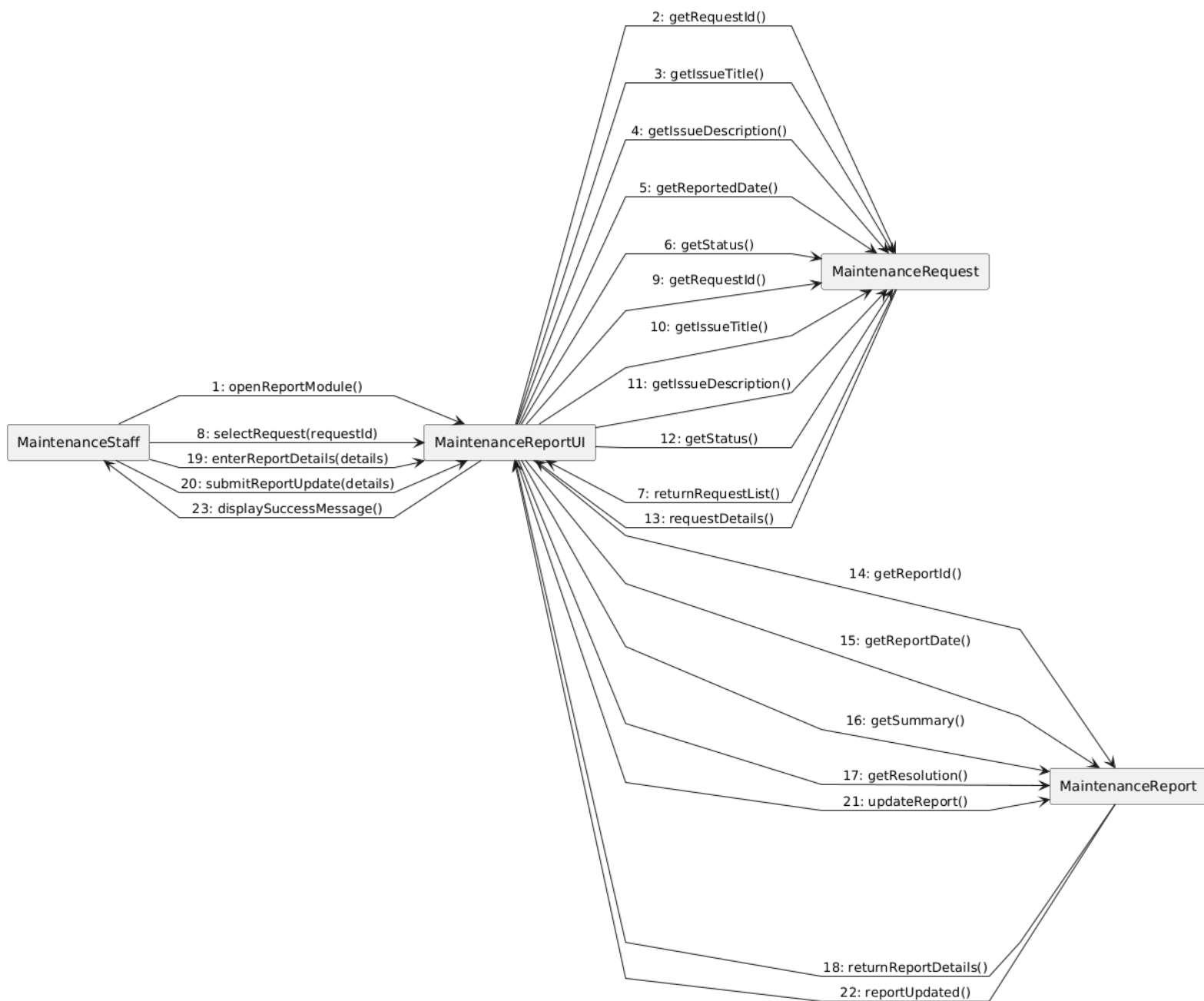
UC-22: Update Maintenance Report - Communication Diagram
